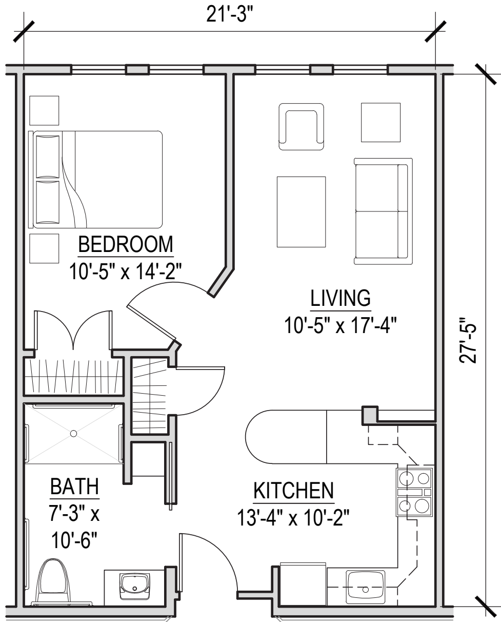
ONE BEDROOM 580 SQUARE FEET
