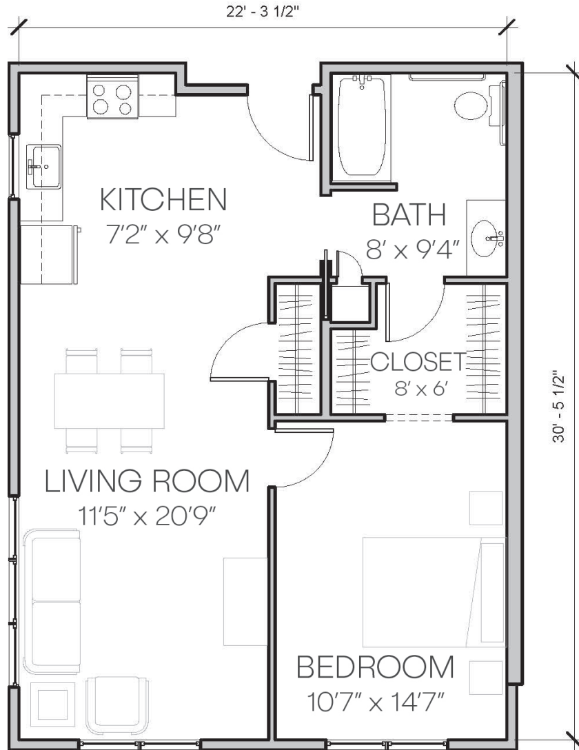
① UNIT B - ONE BEDROOM 3/16" = 1'-0"
